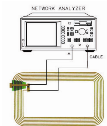
Figure 3. The diagram of antenna impedance measurement
